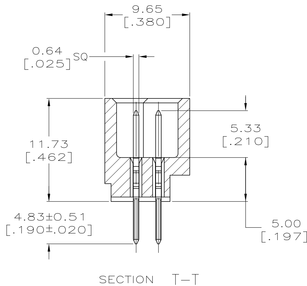
SECTION T-T
