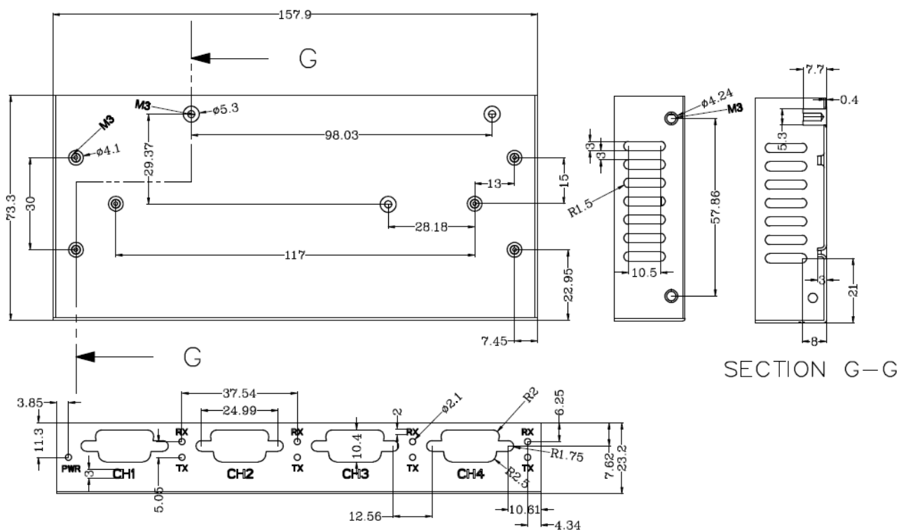
Figure 7.6 - USB2-H-5004-M Bottom Cover of Dimension
