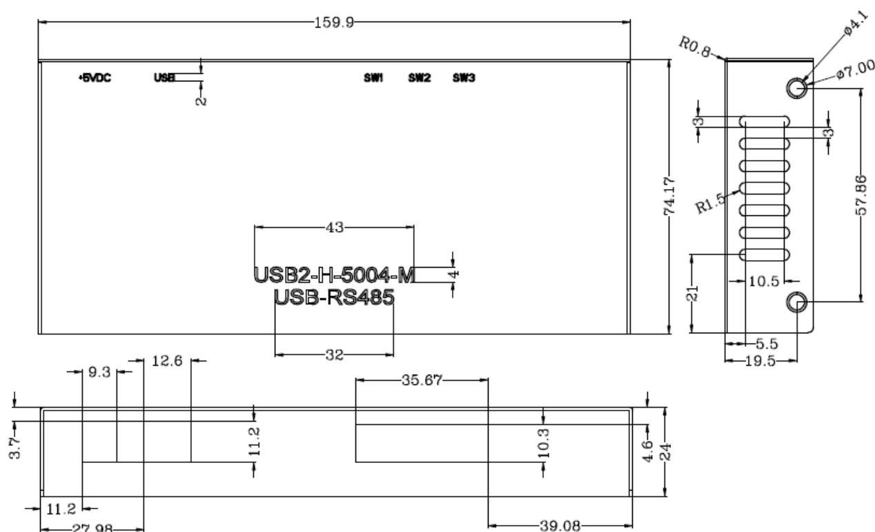
Figure 7.5 - USB2-H-5004-M Top Cover of Dimension
