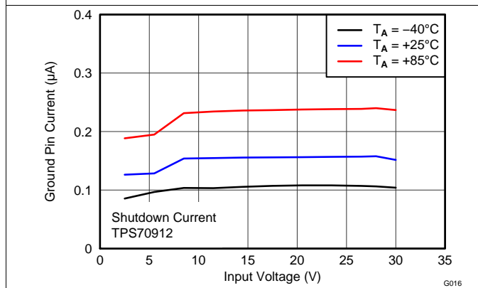
Figure 15. GND Current vs V_{IN} and Temperature
