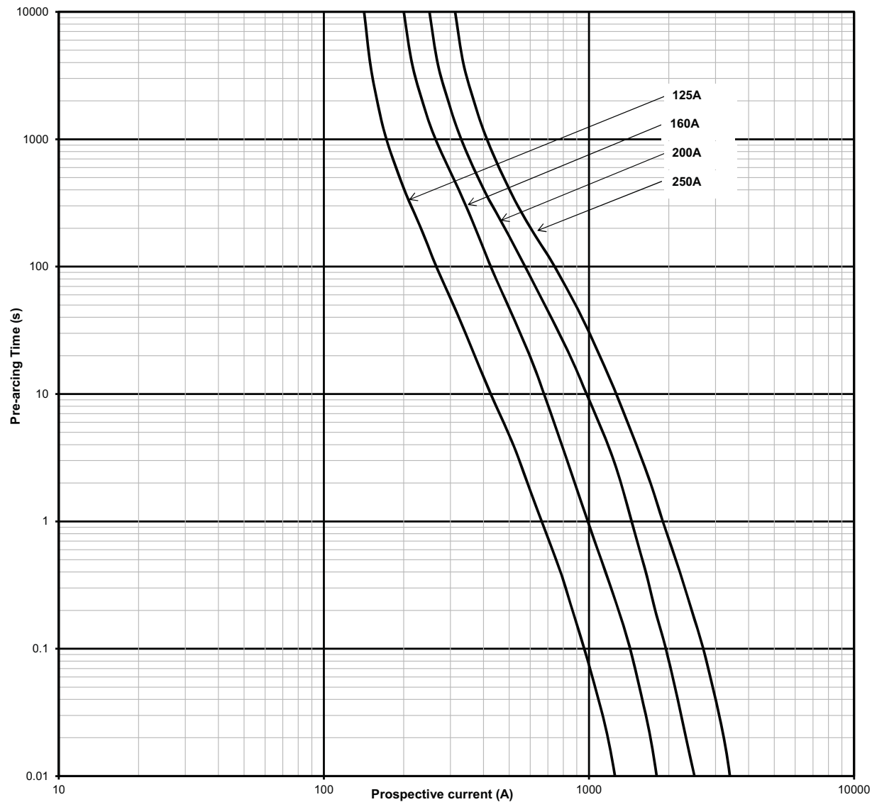
Time current curve - 1500 V d.c.- 2XL - Bladed and bolted
