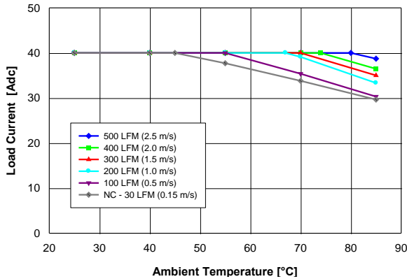
Figure 1.2V.9. Available load current vs. ambient air temperature and airflow rates for QME48T40012 converter with G height pins mounted vertically with air flowing from pin 1 to pin 3, MOSFET temperature \leq 120\text{ }^{\circ}\text{C} , V_{in} = 48\text{ V} .
