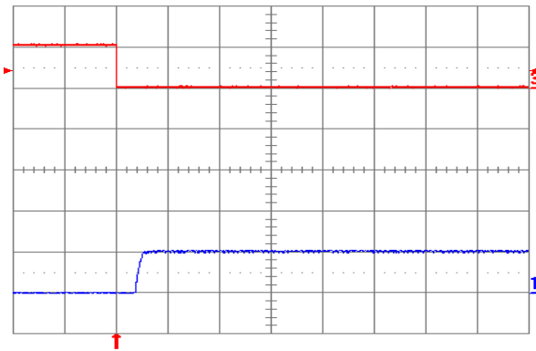
Figure 1.0V.15. Turn-on transient at full rated load current (resistive) with no output capacitor at V_{in} = 48\text{ V} , triggered via ON/OFF pin. Top trace: ON/OFF signal (5 V/div.). Bottom trace: output voltage (1 V/div.). Time scale: 2 ms/div
