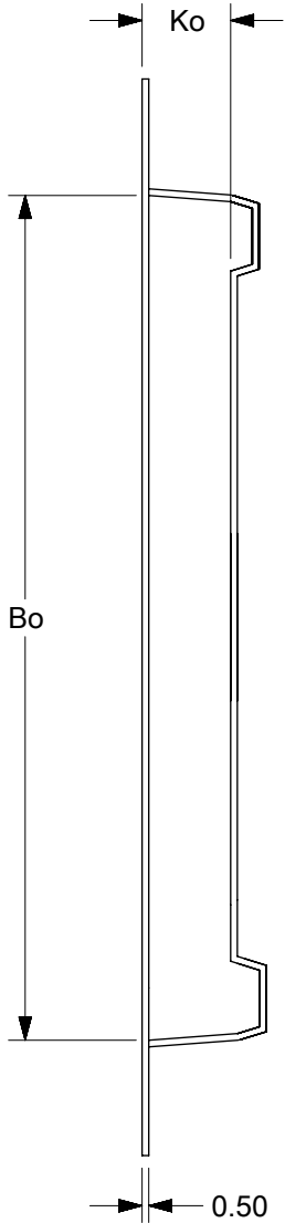
SECTION X-X
