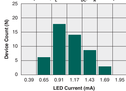
1-Form-A Typical I_F for Switch Dropout (N=50, I_L=100\text{mA}_{\text{DC}} , T_A=25^\circ\text{C} )
