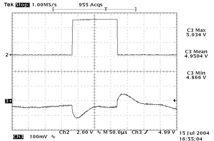
Figure 24: Typical transient response to step load change at 10A/µs from 50% to 75% and 75% to 50% of I_o , max at 12Vin, 5.0V out
