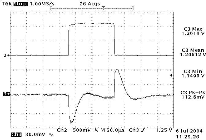
Figure 19: Typical transient response to step load change at 10A/µs from 50% to 75% and 75% to 50% of I_o , max at 12Vin, 1.2V out
