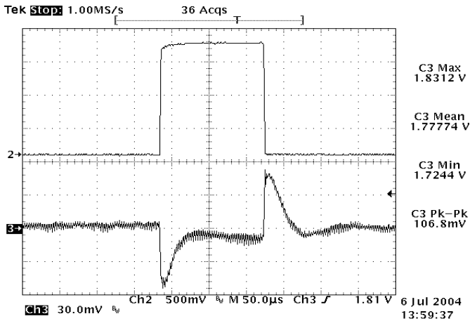
Figure 21: Typical transient response to step load change at 10A/µs from 50% to 75% and 75% to 50% of I_o , max at 12Vin, 1.8V out
