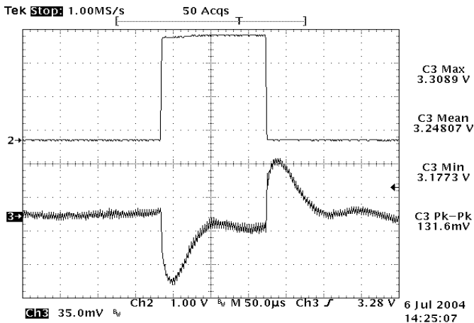
Figure 23: Typical transient response to step load change at 10A/µs from 50% to 75% and 75% to 50% of I_o , max at 12Vin, 3.3V out
