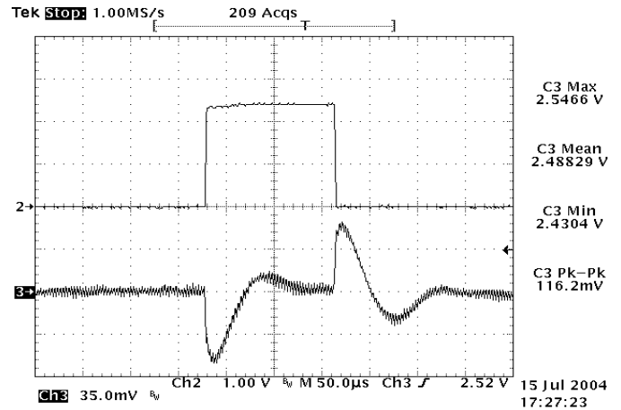
Figure 22: Typical transient response to step load change at 10A/µs from 50% to 75% and 75% to 50% of I_o , max at 12Vin, 2.5V out
