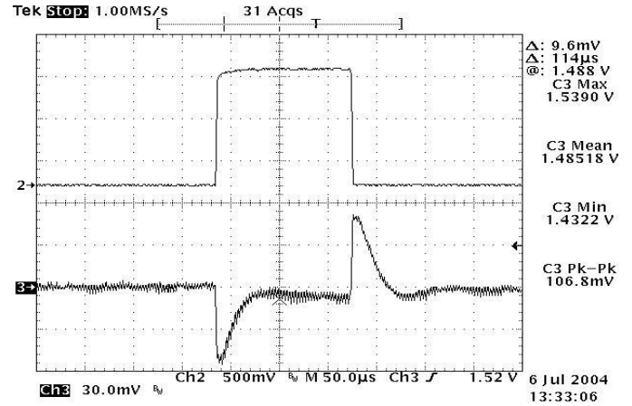
Figure 20: Typical transient response to step load change at 10A/µs from 50% to 75% and 75% to 50% of I_o , max at 12Vin, 1.5V out
