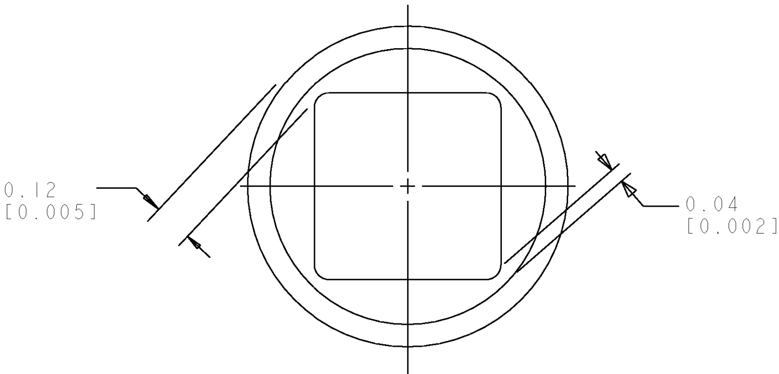
⚠ SOLDER TERMINATION AREA SCALE 40:1 RECOMMENDED PRINTED CIRCUIT SOLDER HOLE FINISHED HOLE: Ø1.02 [.040] ±.08 [.003] DRILLED HOLE: Ø1.15 [.0453] ±.013 [.0005] COPPER PLATE: .025 [.0010] MIN. TIN PLATE: .008 [.0003] MIN. (PER SURFACE)
