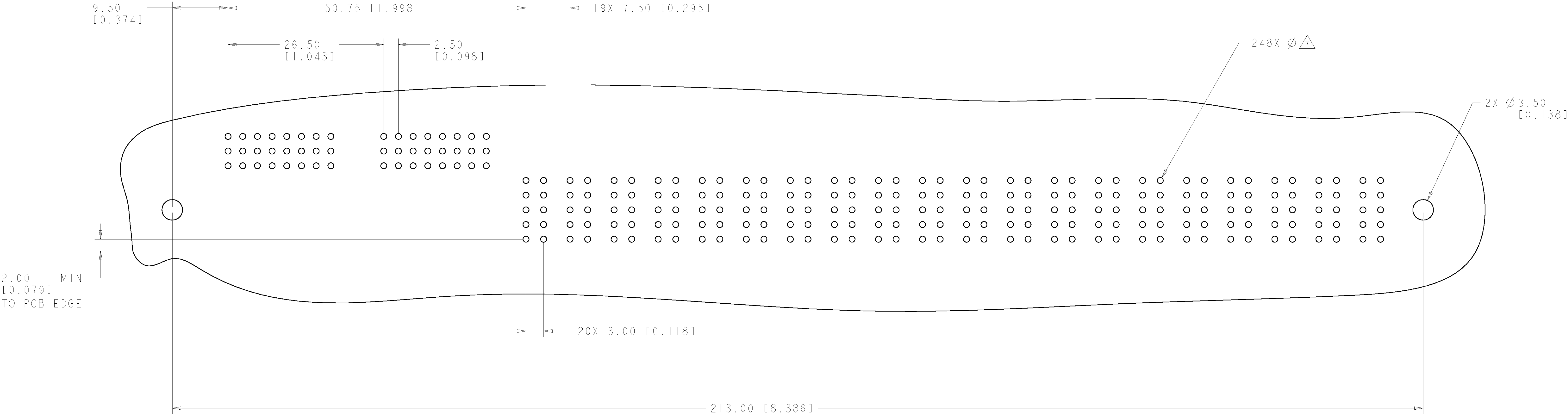
PRINTED CIRCUIT LAYOUT COMPONENT SIDE
