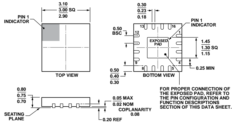
Figure 68. 16-Lead Lead Frame Chip Scale Package [LFCS] 3 mm x 3 mm Body and 0.75 mm Package Height (CP-16-21)
