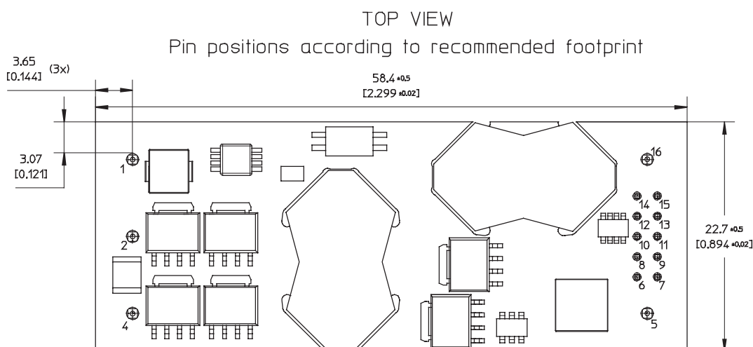
RECOMMENDED FOOTPRINT - TOP VIEW
