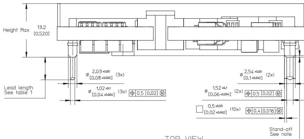
TOP VIEW
