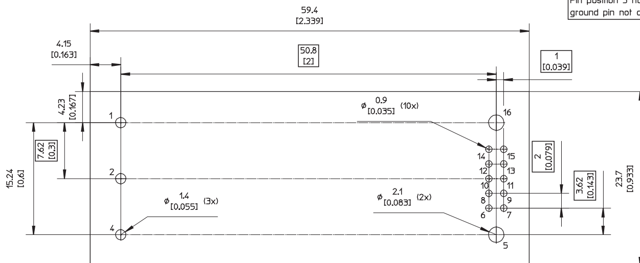
RECOMMENDED FOOTPRINT - TOP VIEW
