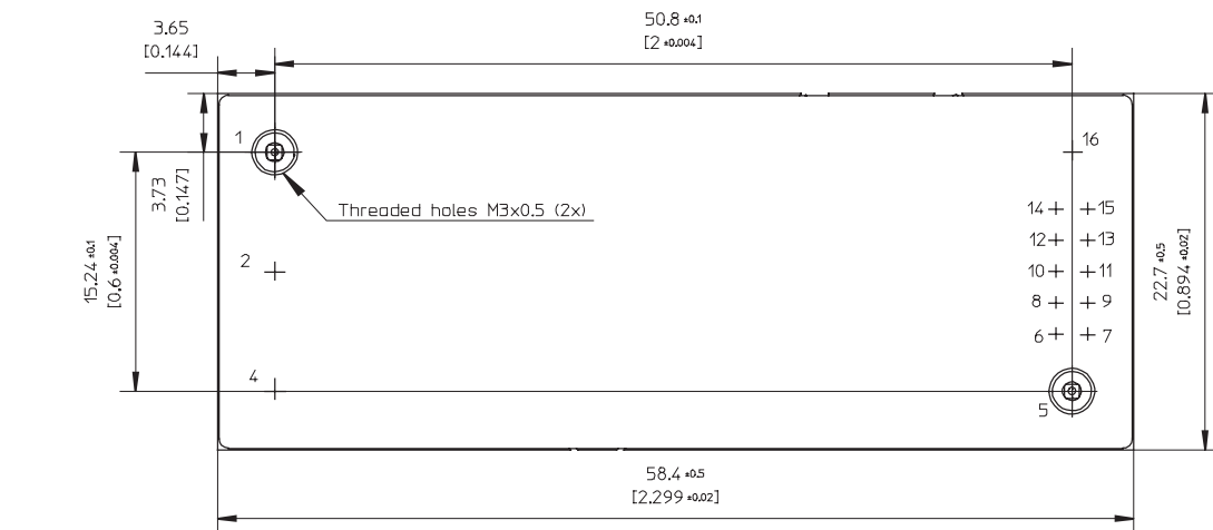
RECOMMENDED FOOTPRINT - TOP VIEW
