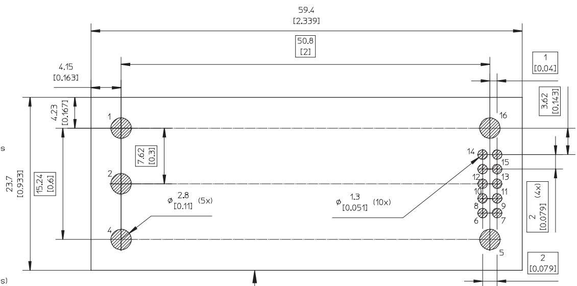
RECOMMENDED FOOTPRINT - TOP VIEW
