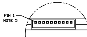
DETAIL B 4X SCALE
