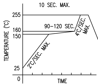
② LEAD FREE REFLOW PROFILE
