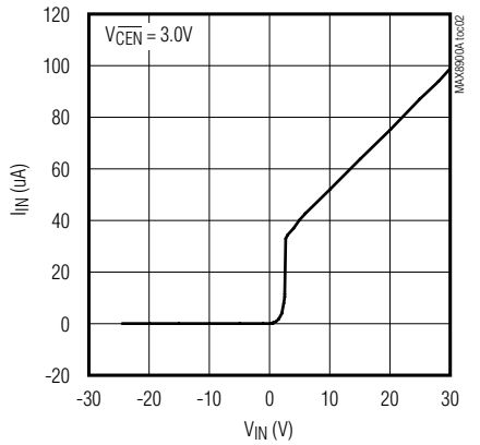
INPUT SUPPLY CURRENT vs. INPUT VOLTAGE ( V_{IN2BAT} DETAIL)
