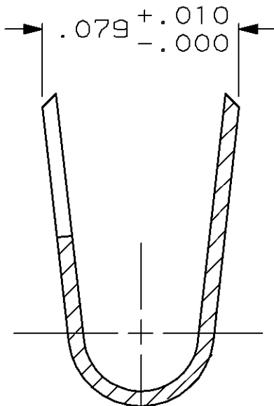
SECT. C-C INSULATION RANGE Ø.035-.060 SCALE 20:1
