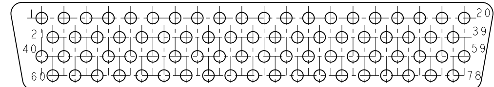
78 POSITION MSI8277-2 SHELL SIZE 5
