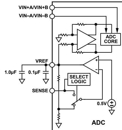
Figure 56. Internal Reference Configuration
