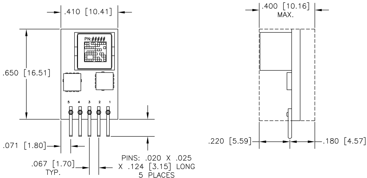
Figure 16. Mechanical Drawing
