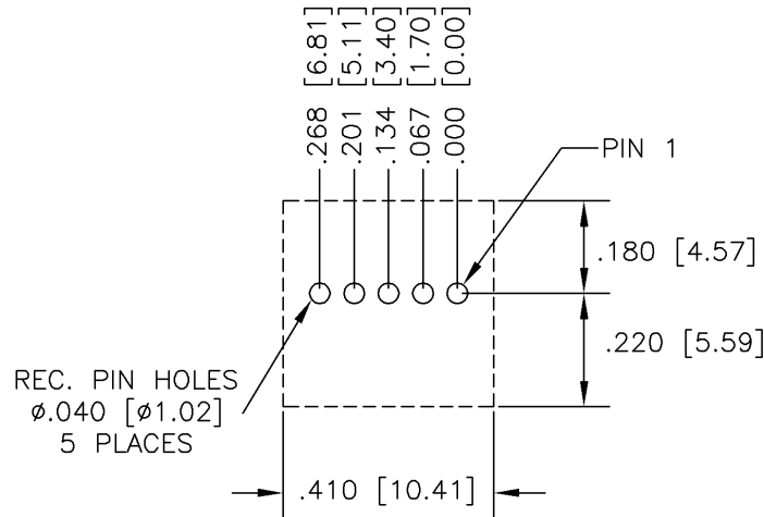
Figure 17. Recommended Footprint – Top View
