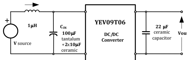
Figure 15. Test Setup for Measuring Input Reflected-Ripple Current and Output Voltage Ripple
