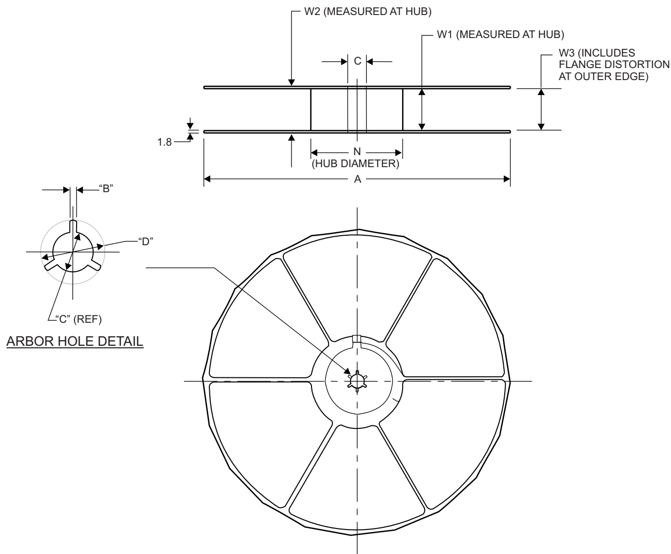
Figure 32. Reel Dimensions
