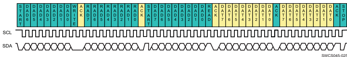
Figure 27. I²C Read Access Multiple Bytes
