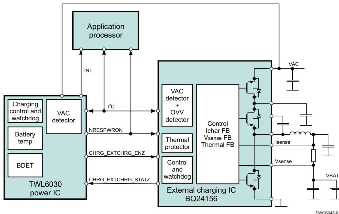
Figure 15. External Charger Interface
