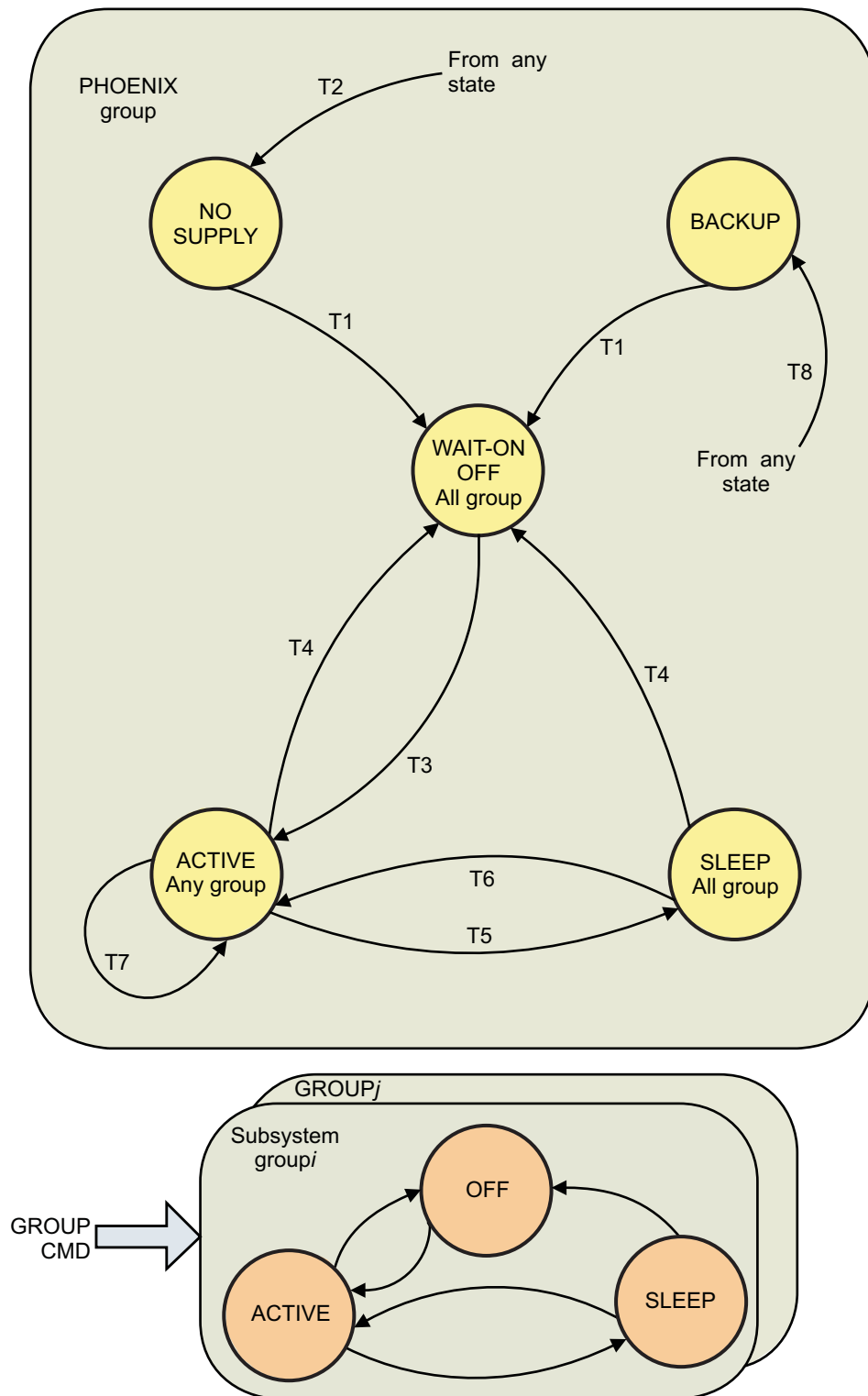
Figure 10. Power-State Transition Diagram
