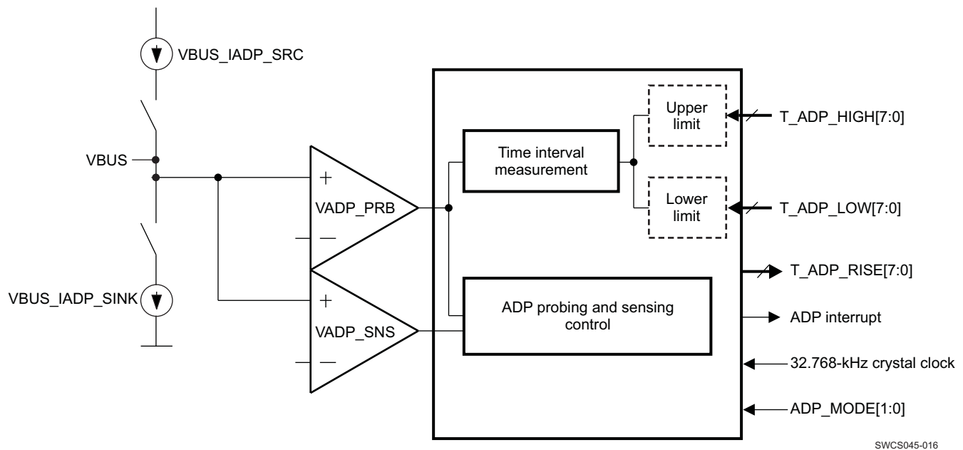
Figure 17. Attach Detection Protocol Scheme
