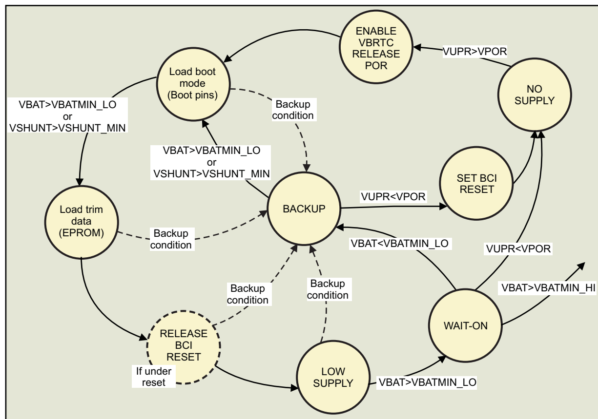
Figure 9. Boot Sequence
