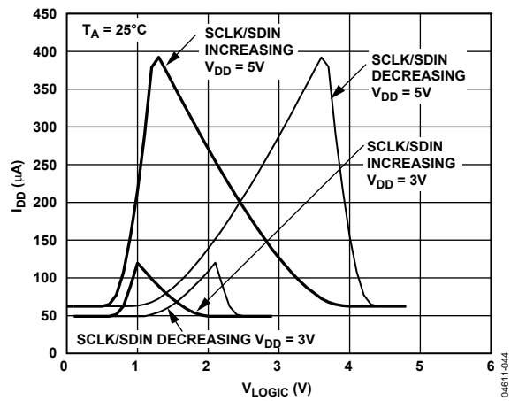
Figure 32. SCLK/SDIN vs. Logic Voltage
