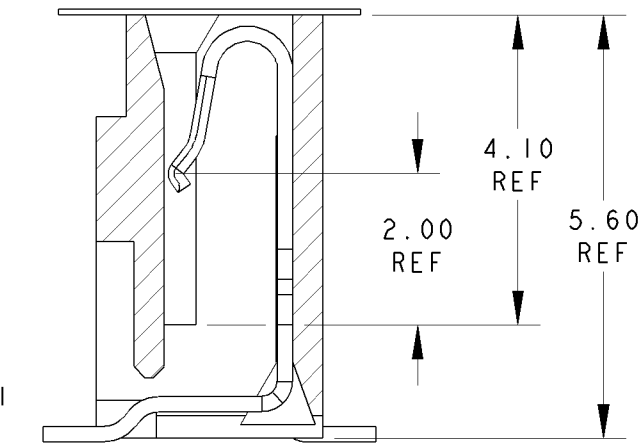
SECTION A-A (FOR EVEN POSITION CONTACTS) SCALE 10:1
