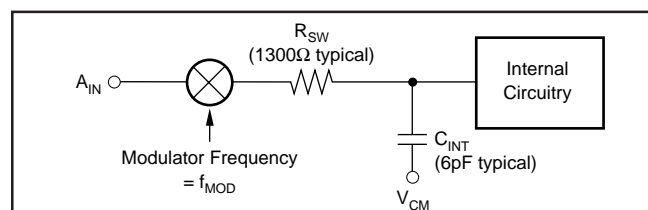
FIGURE 1. Analog-Input Structure.
