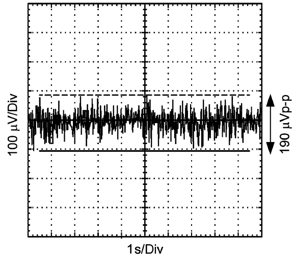
Figure 20. 0.1–10 Hz Noise
