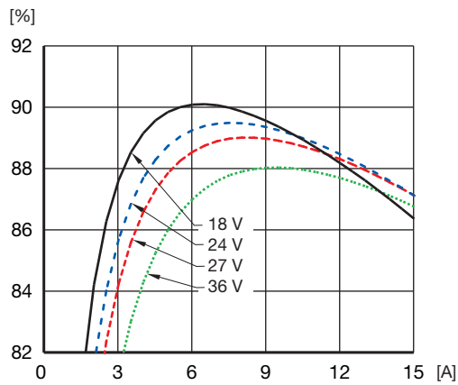
Efficiency vs. load current and input voltage at T_{Pcb}=+25\text{ }^{\circ}\text{C}
