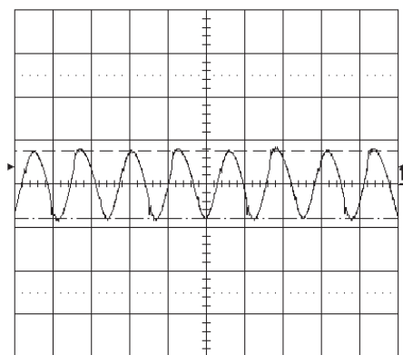
Output voltage ripple (50mV/div.) at T_{Pcb}=+25 °C, V_{in}=27 V, I_o=4.2 A resistive load with C=10 μF tantalum and 0.1 μF ceramic capacitors. Band width=20MHz. Time scale: 2 μs / div.
