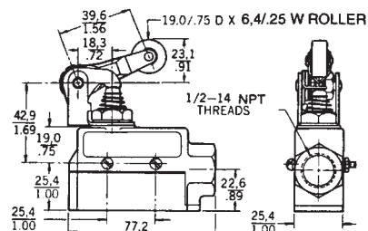
Side mount without seal boot
