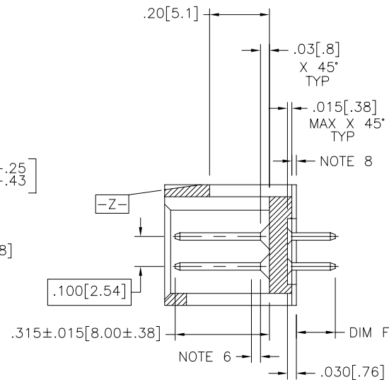
SECTION H-H
