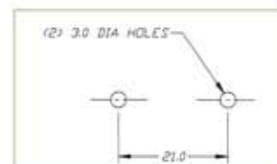
PANEL MOUNT
