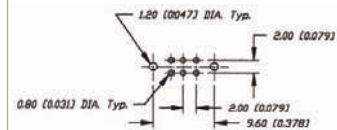
P.C. MOUNTING
