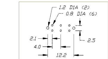
P.C. MOUNTING
