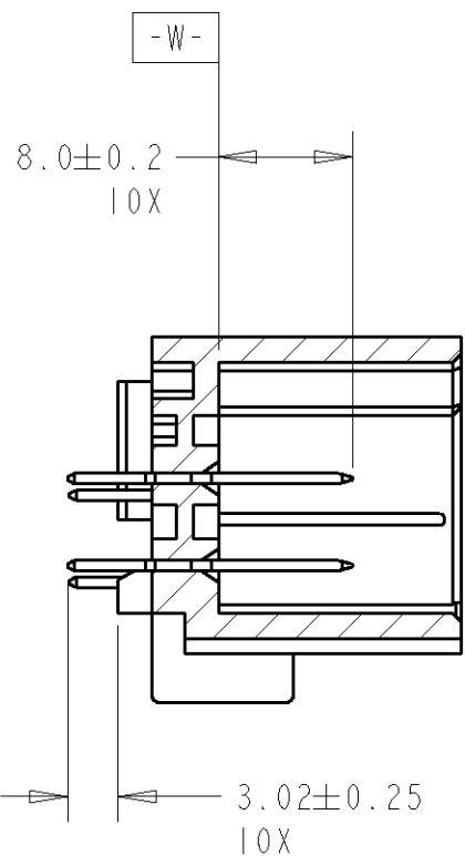
SECTION DD-DD (.070 TABS)
