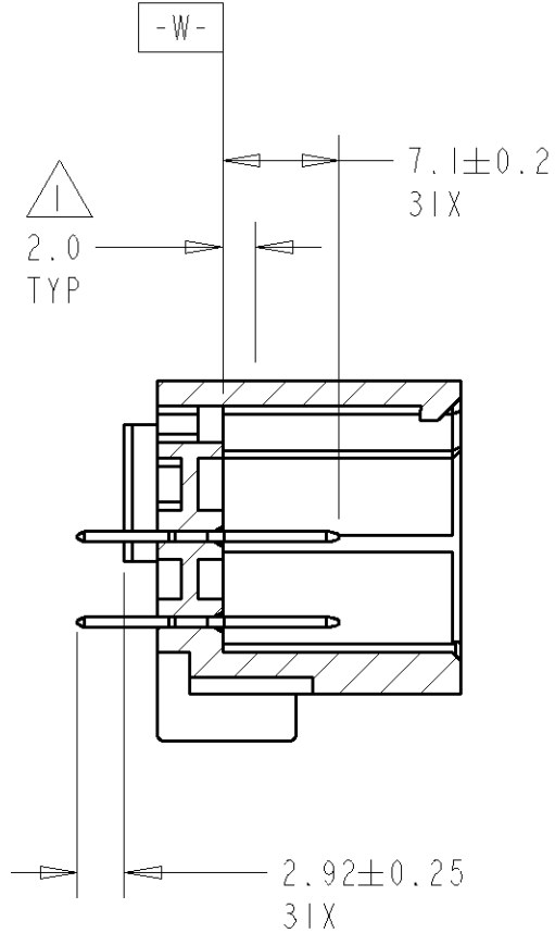
SECTION CC-CC (.040 TABS)
