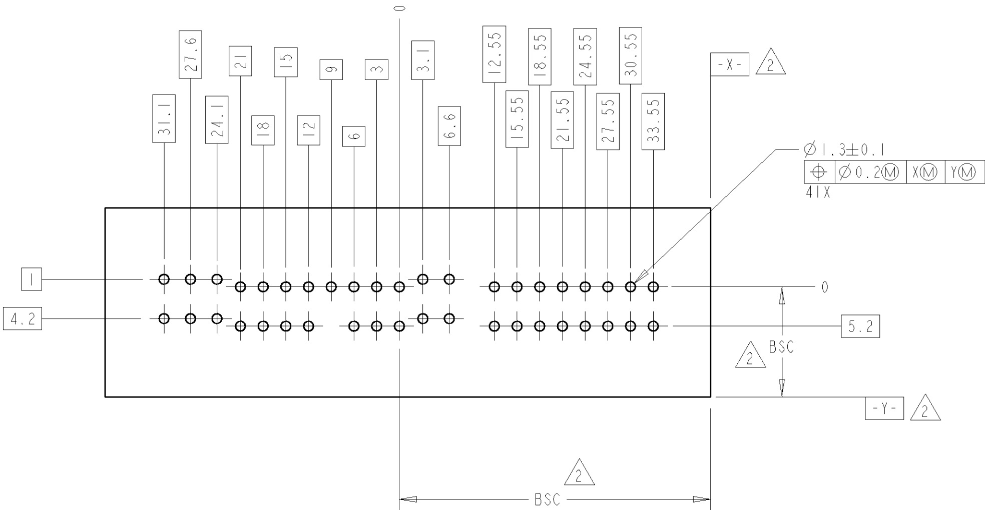
PC BOARD LAYOUT -COMPONENT SIDE (RECOMMENDED BOARD THICKNESS 1.57mm) SCALE 2:1
