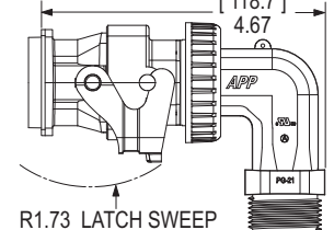
Mated Side View
