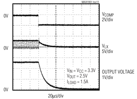
SHUTDOWN WAVEFORMS
