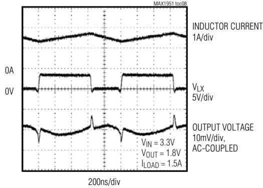
SWITCHING WAVEFORMS
