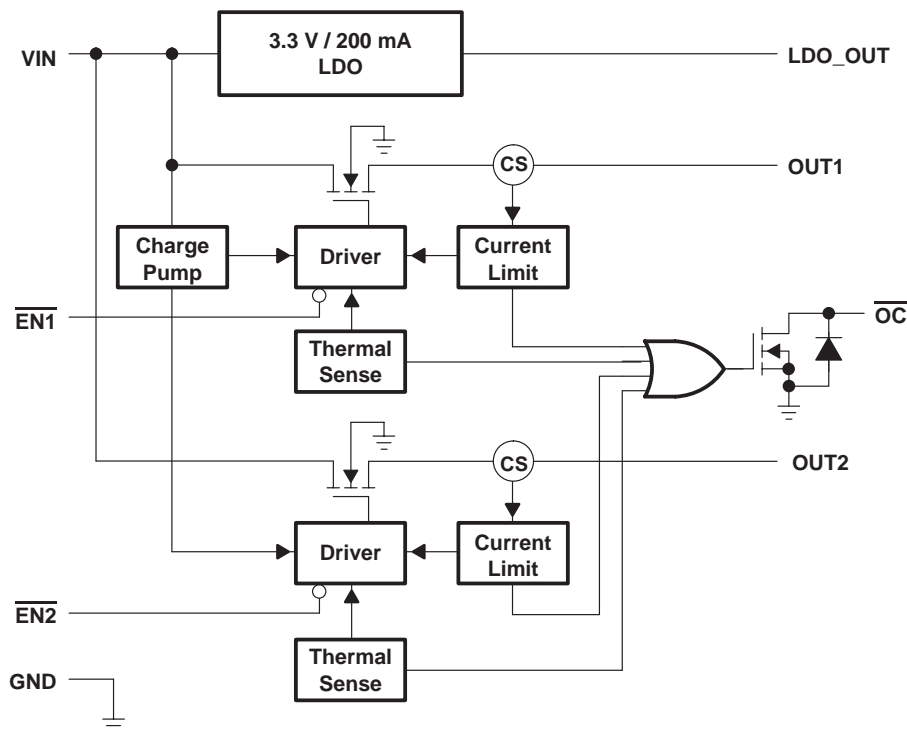
Terminal Functions
