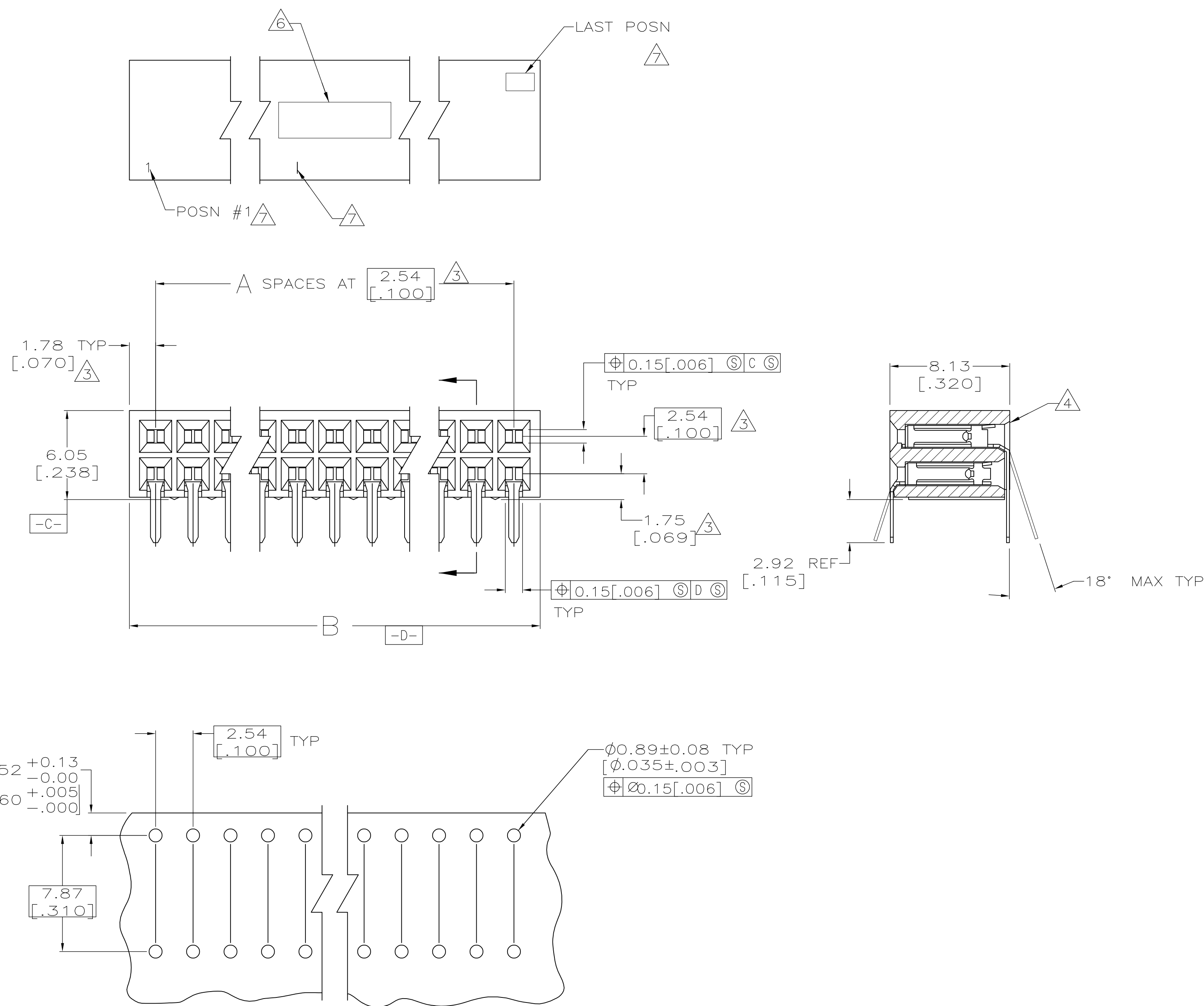
RECOMMENDED PC BOARD HOLE LAYOUT
