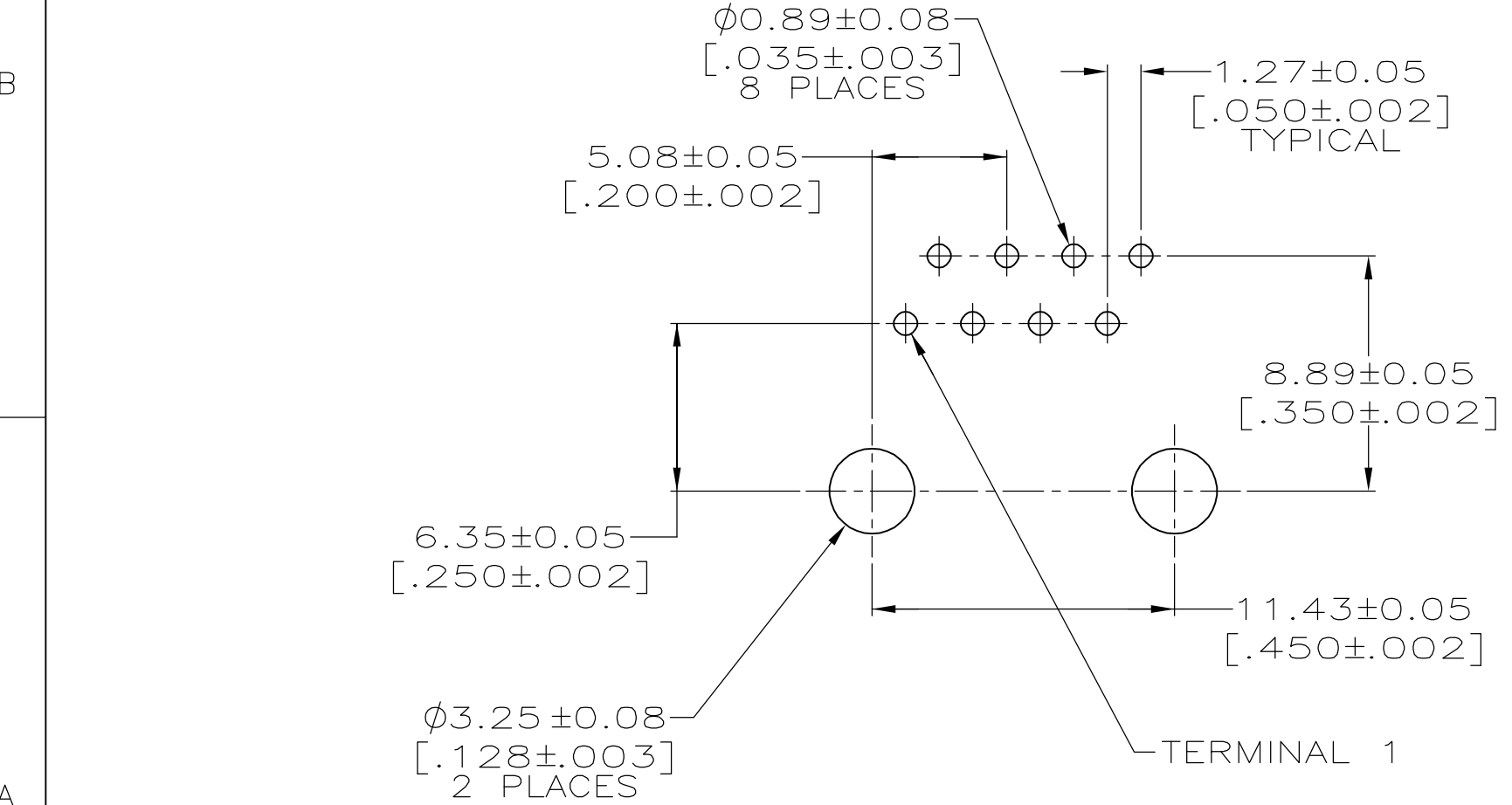
SUGGESTED PC BOARD LAYOUT COMPONENT SIDE SCALE 4:1
