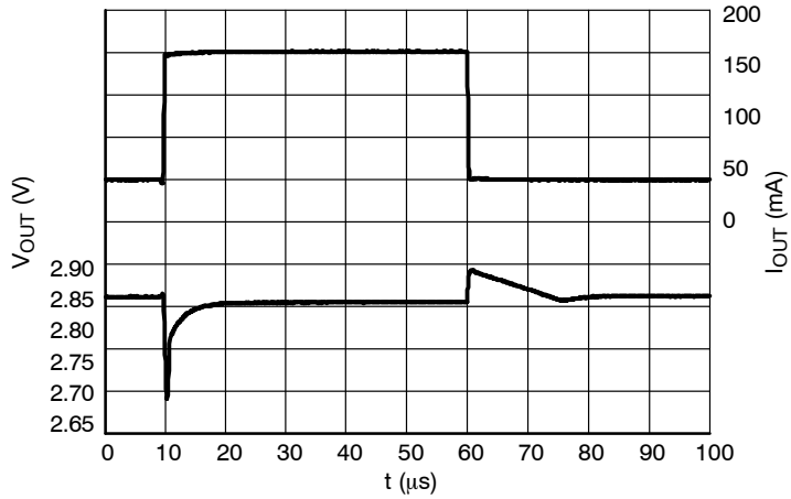
Figure 34. Load Transients, 2.8 V Version, I OUT = 1 – 150 mA, t R = t F = 0.5 μs, V IN = 3.8 V
