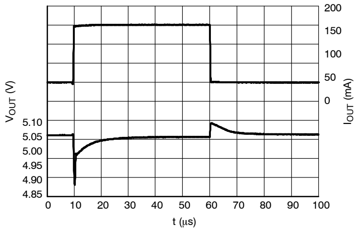
Figure 35. Load Transients, 5.0 V Version, I OUT = 1 – 150 mA, t R = t F = 0.5 μs, V IN = 6.0 V
