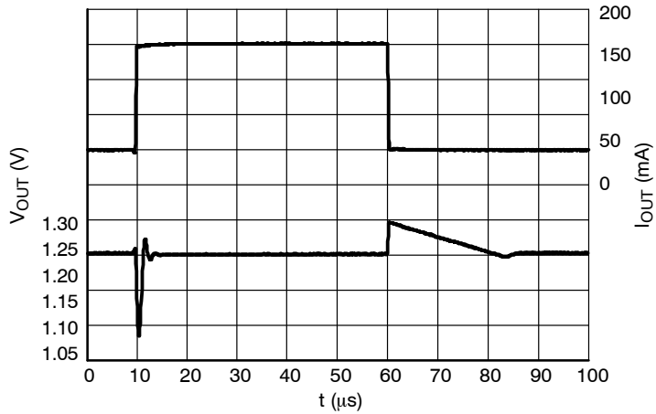
Figure 33. Load Transients, 1.2 V Version, I OUT = 1 – 150 mA, t R = t F = 0.5 μs, V IN = 2.2 V
