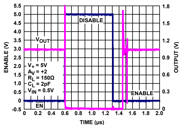
FIGURE 12. ENABLE/DISABLE TIMING
