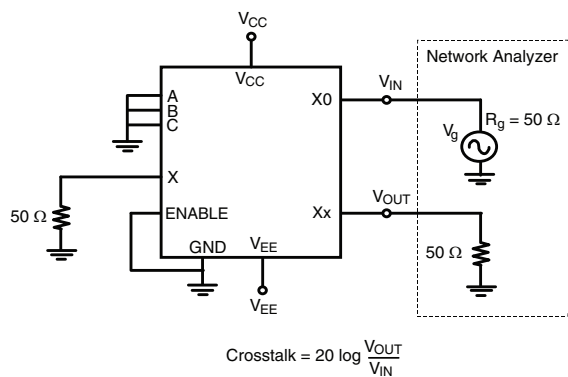
Fig. 6 - Crosstalk
