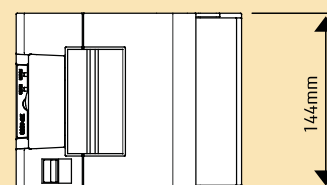
Standard Model
