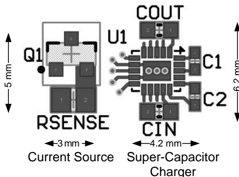
Figure 72. LM3550 Layout
