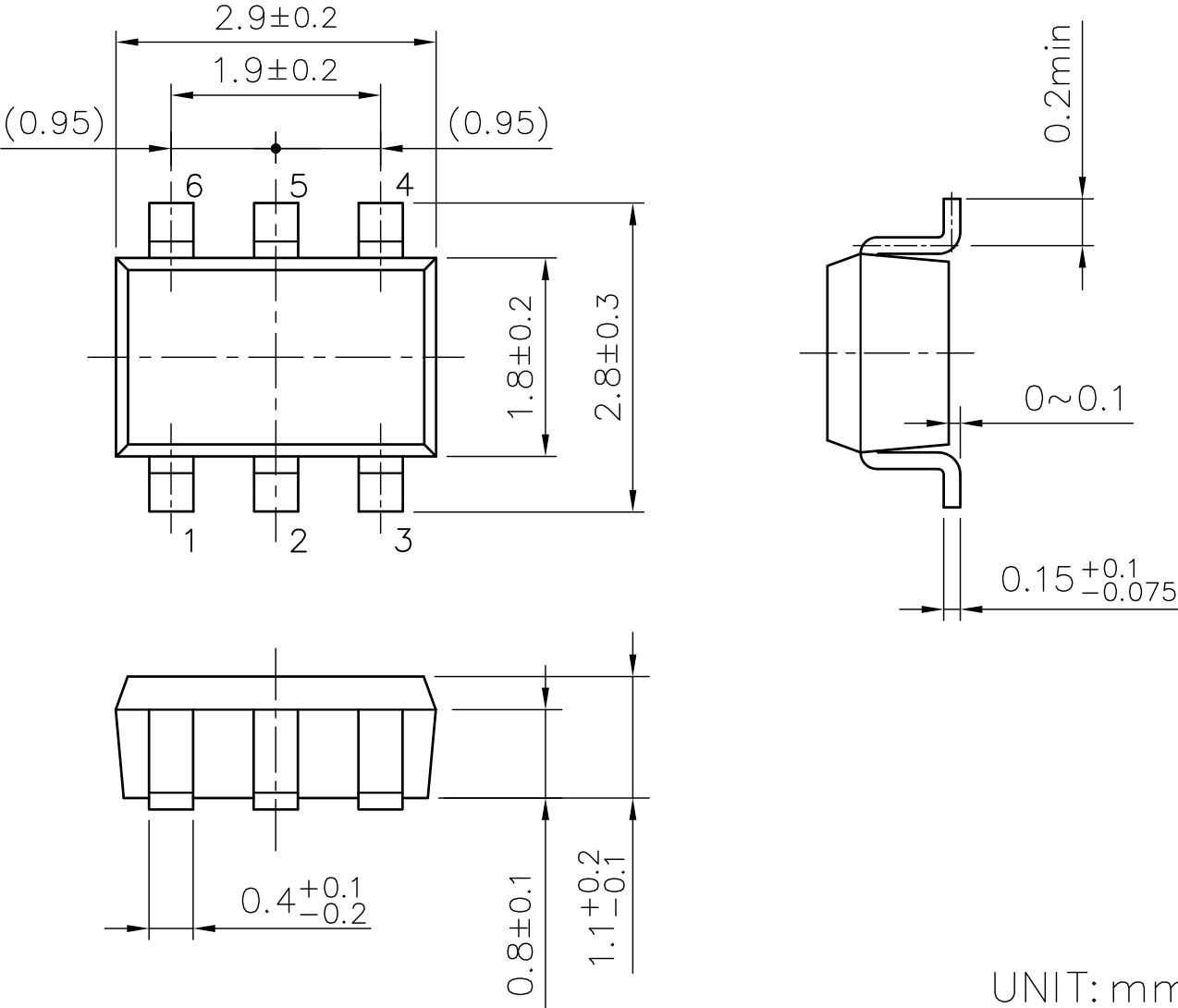
SOT-23-6W Package Dimensions (Unit: mm)
