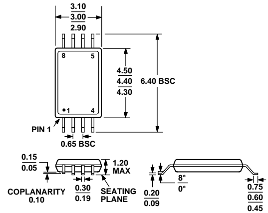
Figure 20. 8-Lead Thin Shrink Small Outline Package [TSSOP] (RU-8) Dimensions shown in millimeters
