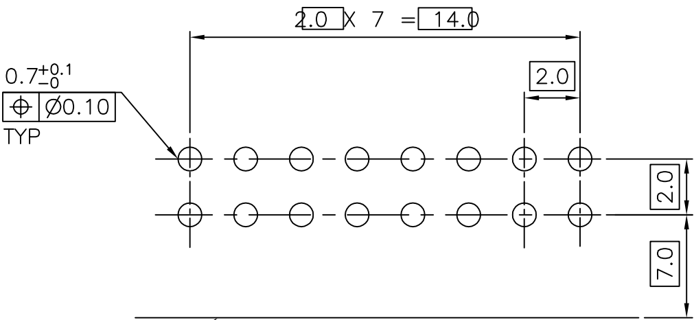
RECOMMENDED PCB LAYOUT (THICKNESS:1.6MM) (TOP VIEW) (TOLERANCE:±0.05)
