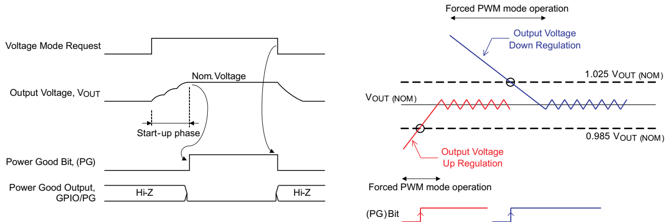
Figure 34. Power Good Operation (DIR = 1, GPIOTYPE = 1)
