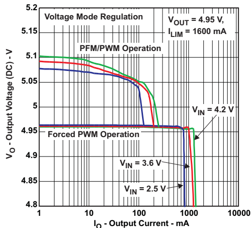
Figure 16. DC Output Voltage vs Load Current
