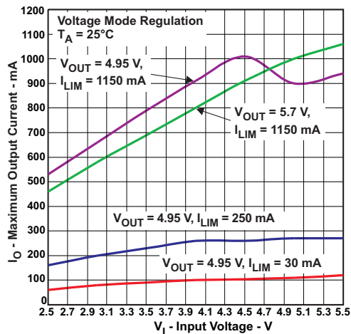
Figure 18. Maximum Output Current vs Input Voltage
