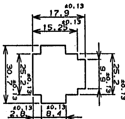
パネル取付穴寸法 FIG. 1 (RECOMMENDED PANEL OPENING DIMENSION)
