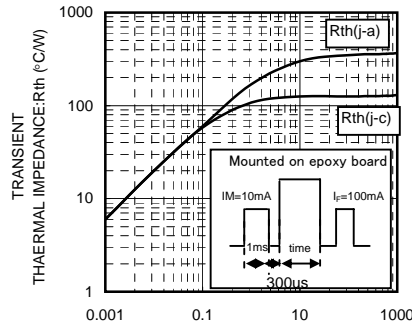
THAERMAL IMPEDANCE: R_{th} (°C/W) R_{th} - t CHARACTERISTICS
