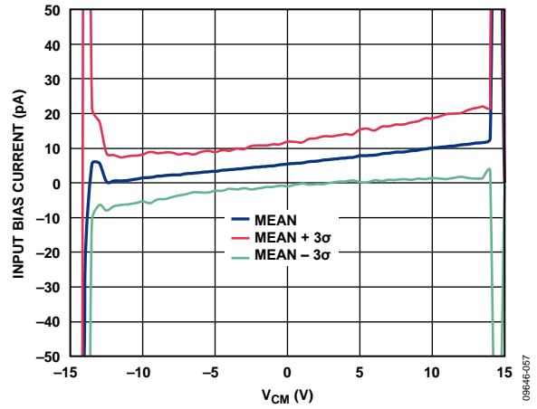
Figure 18. Input Bias Current vs. Common-Mode Input Voltage ( V_{CM} ), Mean and Three Standard Deviations, V_{SY} = \pm 15 V, R_L = \infty
