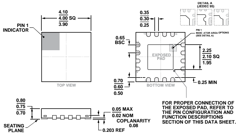
Figure 69. 16-Lead Lead Frame Chip Scale Package [LFCSP] 4 mm x 4 mm Body and 0.75 mm Package Height (CP-16-23)
