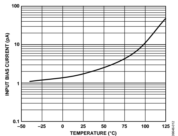
Figure 20. Input Bias Current vs. Temperature, V_{SY} = \pm 15 V
