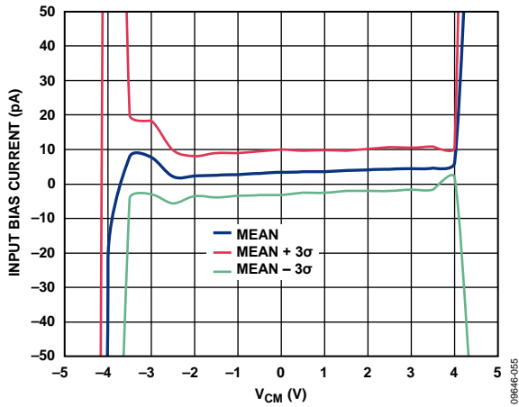
Figure 15. Input Bias Current vs. Common-Mode Input Voltage ( V_{CM} ), Mean and Three Standard Deviations, V_{SY} = \pm 5 V, R_L = \infty
