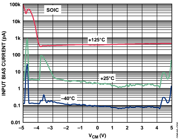
Figure 16. Input Bias Current vs. Common-Mode Input Voltage ( V_{CM} ), Three Temperatures, V_{SY} = \pm 5 V, R_L = \infty
