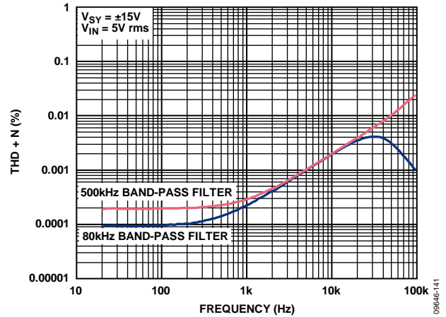
Figure 47. THD + N vs. Frequency, V_{SY} = \pm 15V
