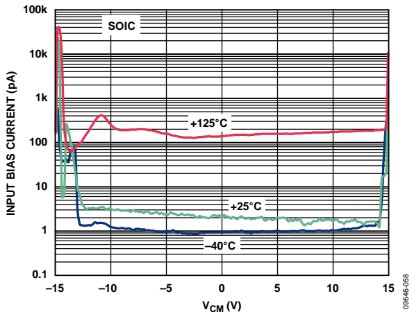
Figure 19. Input Bias Current vs. Common-Mode Input Voltage ( V_{CM} ), Three Temperatures, V_{SY} = \pm 15 V, R_L = \infty
