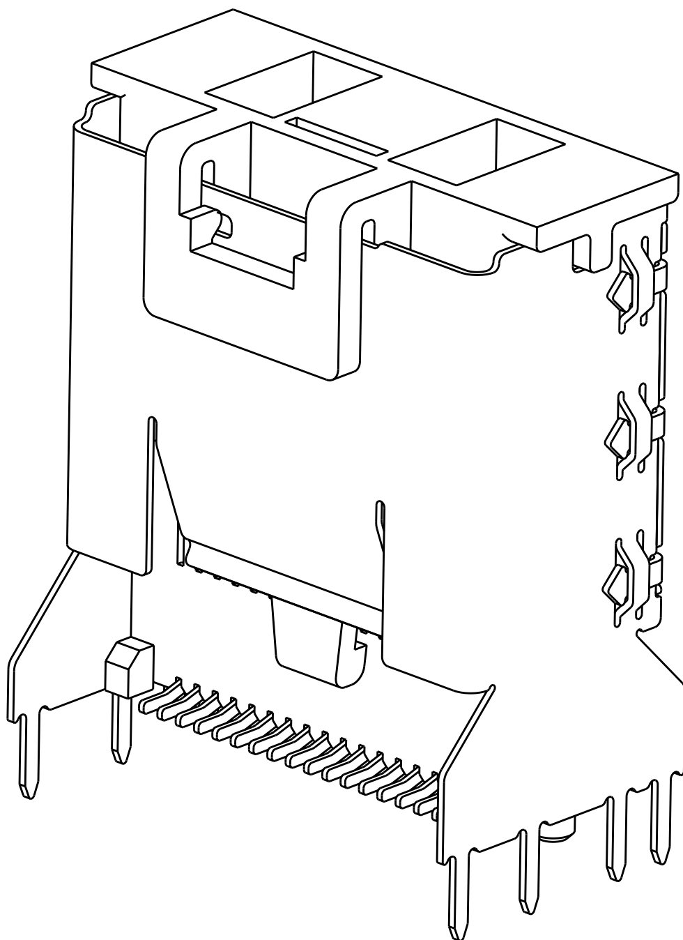
1888863-4 SCALE 6:1
