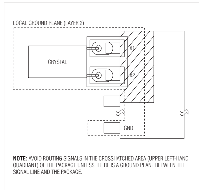
Figure 2. Layout Example
