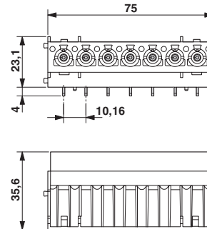
Dimensional drawing
