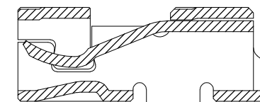
A-A (P/N1827395-2)
