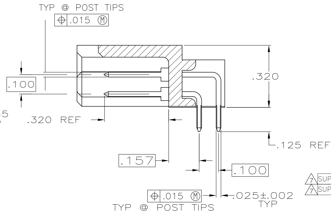
SECTION M-M
